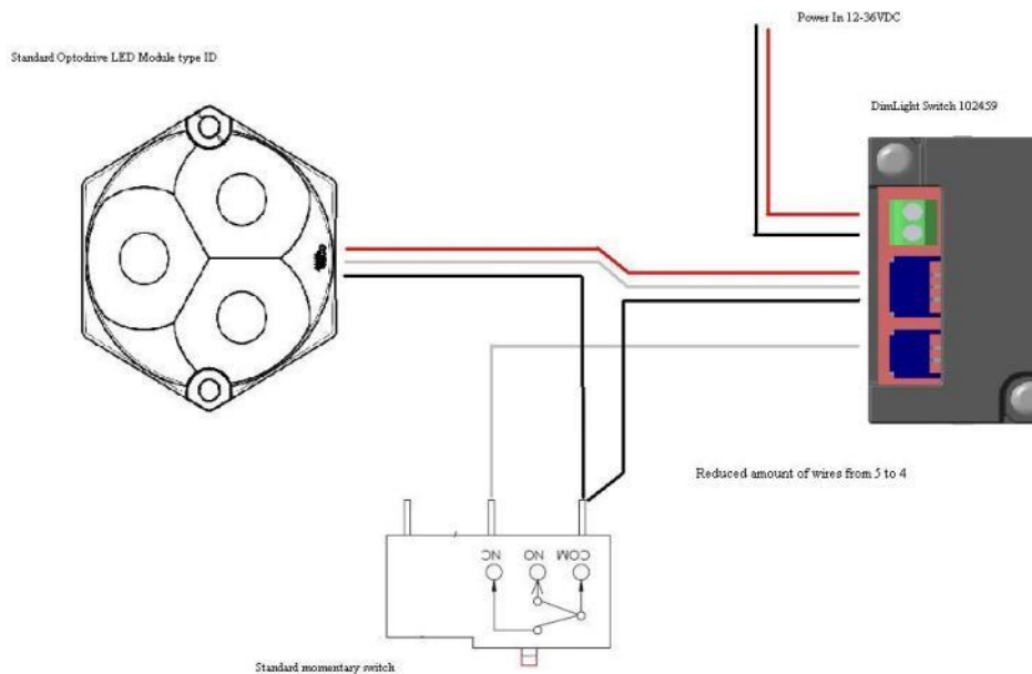
Standard Wire DimLight Switch
